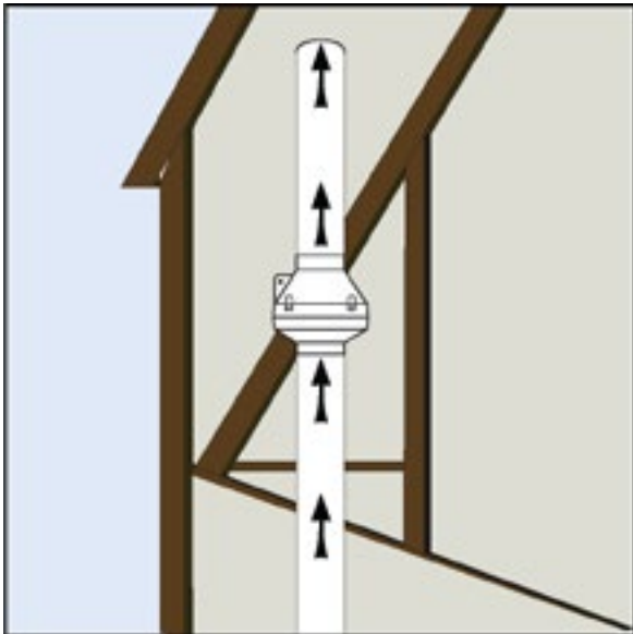
Interior Installation
