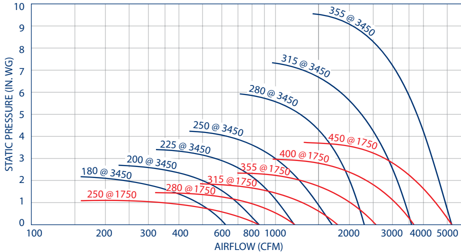
60 Hz DIRECT DRIVE AIRFLOW PERFORMANCE SHOWN USING INLET CONE & SCROLL
