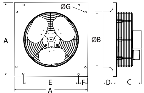
PEF Panel Mount Fans
