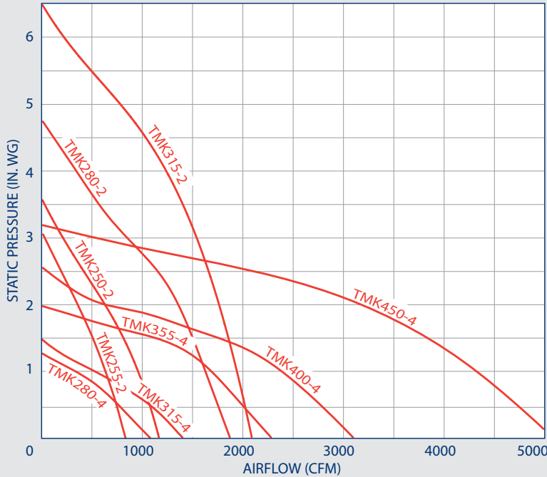
TYPICAL PERFORMANCE (VARIES BY MODEL & VOLTAGE)
