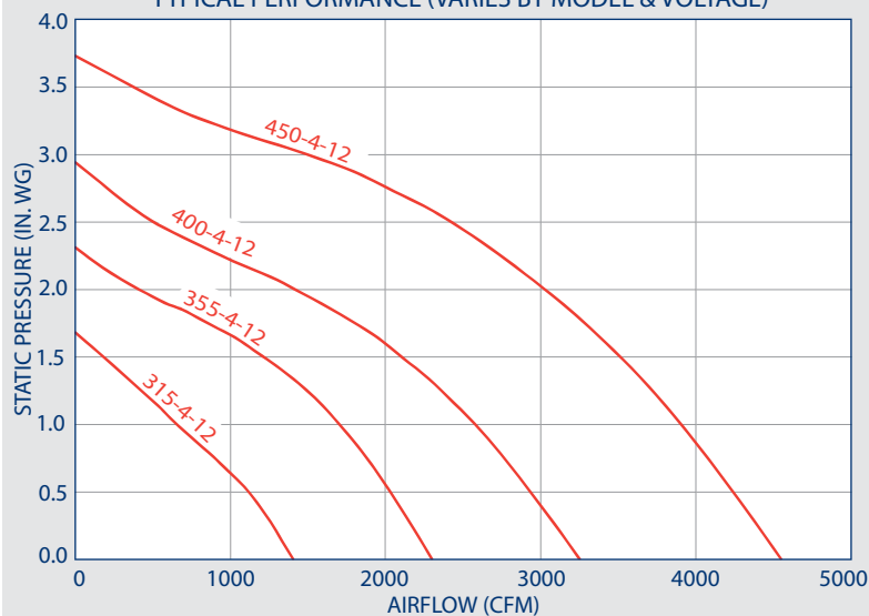
TYPICAL PERFORMANCE (VARIES BY MODEL & VOLTAGE)
