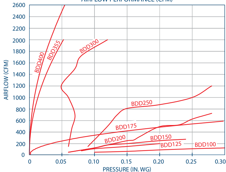
AIRFLOW PERFORMANCE (CFM)
