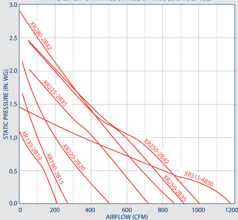
TYPICAL PERFORMANCE (VARIES BY MODEL & VOLTAGE)
