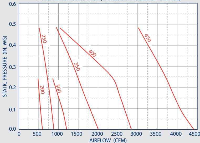
TYPICAL PERFORMANCE (VARIES BY MODEL & VOLTAGE)
