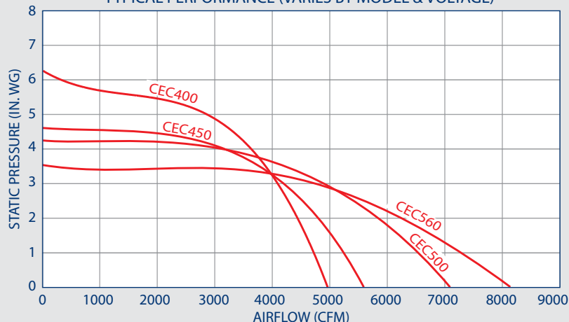
TYPICAL PERFORMANCE (VARIES BY MODEL & VOLTAGE)
